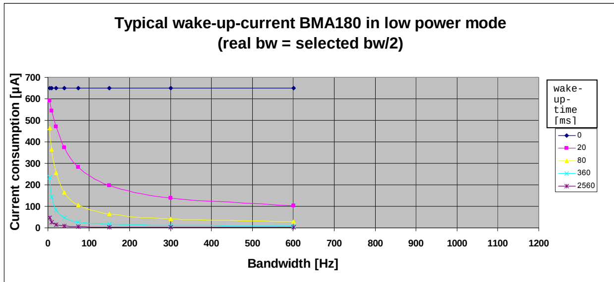
Figure 2: Typical average current consumption in wake-up mode using high-g or low-g interrupt; here typical values in low power mode
