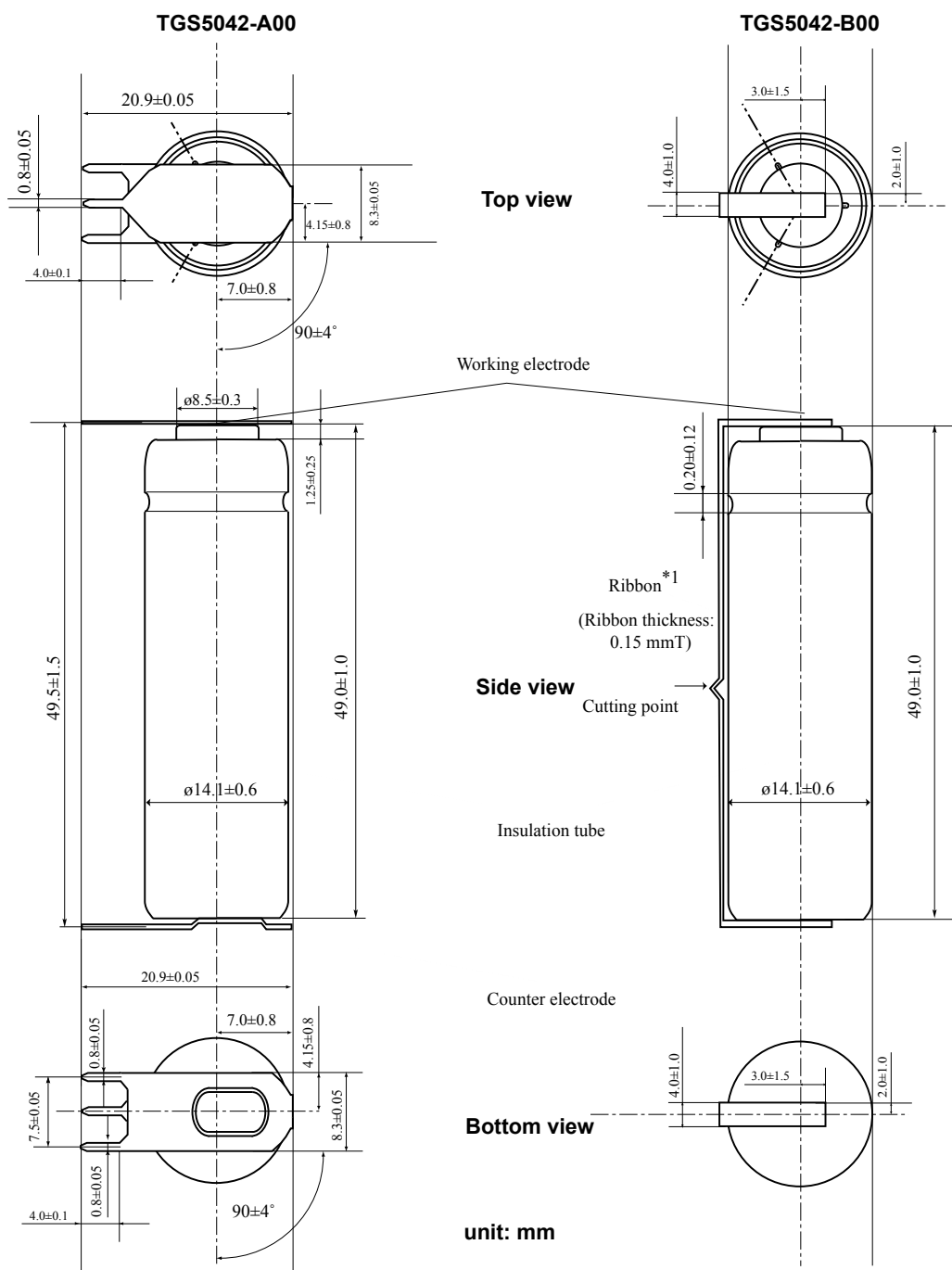
Figure 23 - TGS5042 Dimensions (lead configurations)
