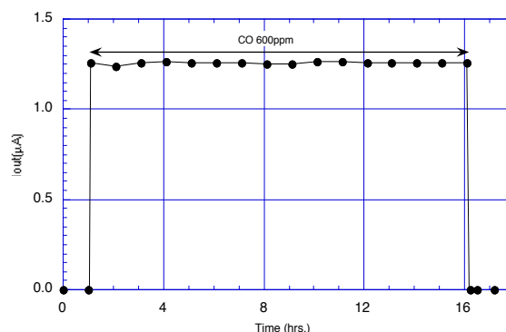
Figure 11a - Normal operation test (CO 600±30ppm for 12 hours at 20°C/40%RH)
