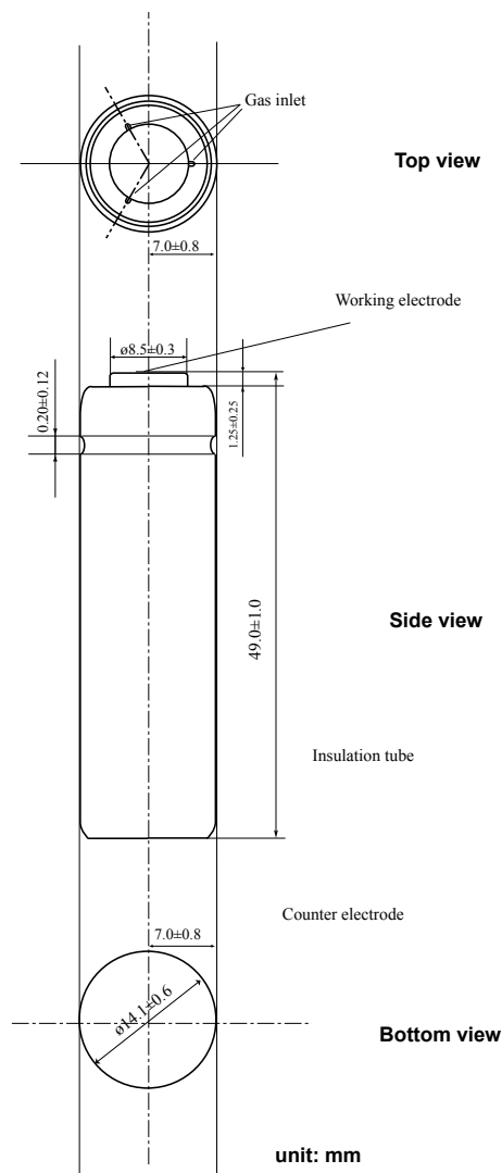
Figure 3 - Dimensions
