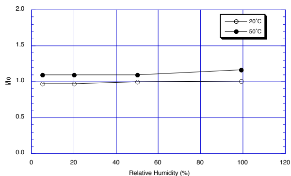
Figure 7b - Humidity dependency at 400ppm CO ( I_o =sensor output current at 50%RH)
