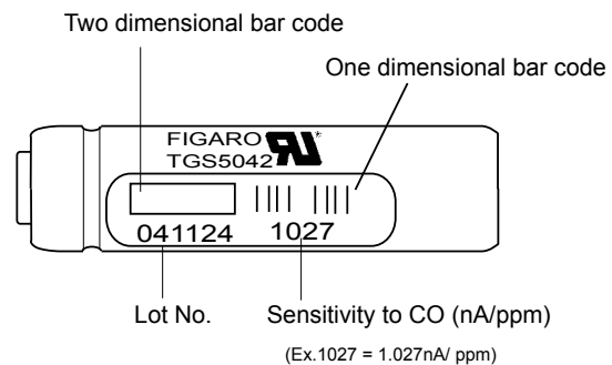
Figure 23 - TGS5042 markings
