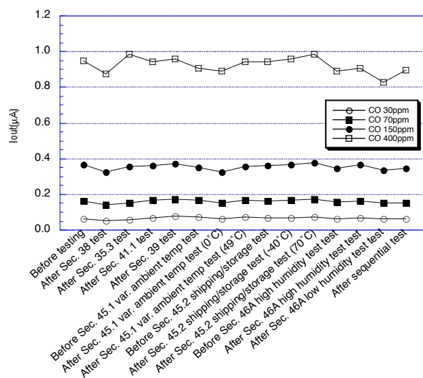
Figure 20 - Sequential test
