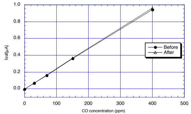
Figure 16b - Effects of shipping and storage
