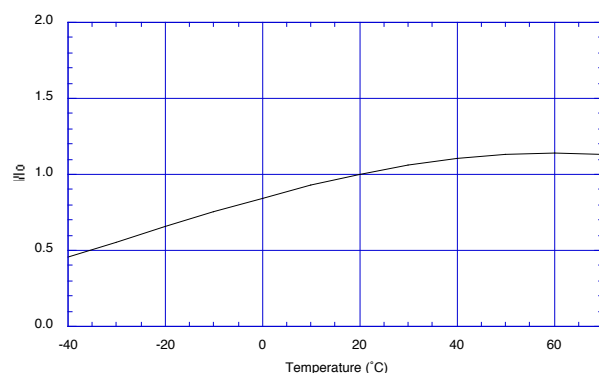
Figure 7a - Temperature dependency at 400ppm CO/50%RH ( I_o =sensor output current at 20°C)
