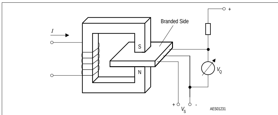
Figure 5 Sensor/Magnetic-Field Configuration
